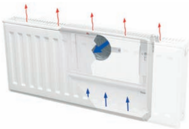
Easy-Vent installed on the wall behind the radiator (in cross-section). The filtered and pre-heated fresh air is supplied to the room at the radiator's upper edge.
